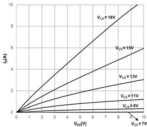
Fig3. Output Characteristics T_j = -40^\circ\text{C}
