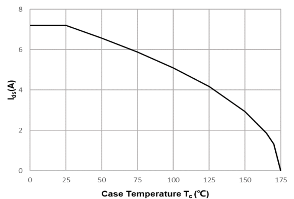
Fig12. Continuous Drain Current vs. Case Temperature
