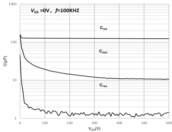
Fig9. Capacitances vs. Drain-Source Voltage (0-600V)
