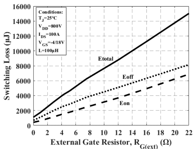
Figure 21. Switching Losses vs. R_{G(ext)}
