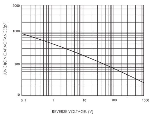
FIG.3-TYPICAL JUNCTION CAPACITANCE
