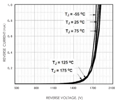
FIG.4-REVERSE CHARACTERISTICS
