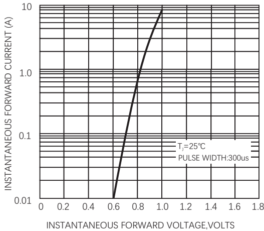
FIG. 3-TYPICAL FORWARD CHARACTERISTICS
