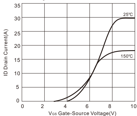
Fig9. Transfer Characteristics
