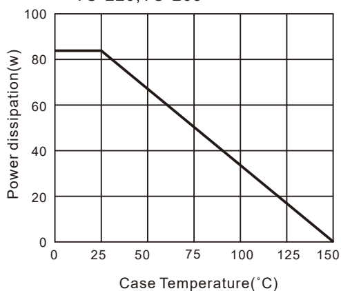
Fig1. Power Dissipation TO-220, TO-263
