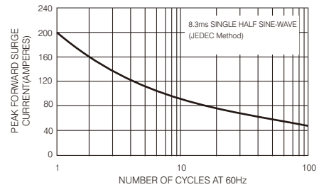
FIG.2-MAXIMUM NON-REPETITIVE FORWARD SURGE CURRENT (Per diode)
