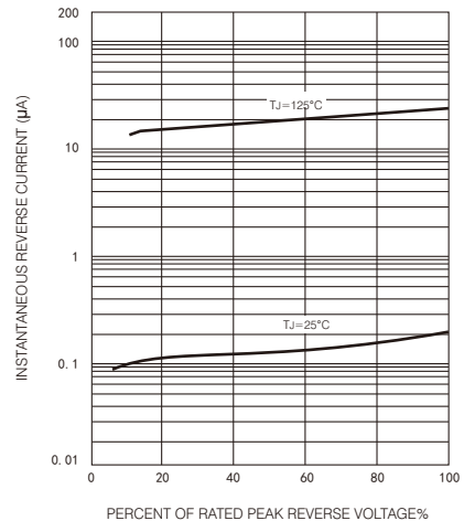
FIG.5-TYPICAL REVERSE CHARACTERISTICS (Per diode)
