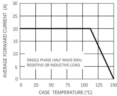
FIG.1-TYPICAL FORWARD CURRENT DERATING CURVE (Per diode)
