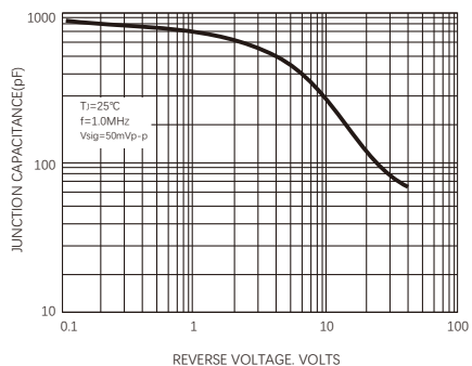
FIG.5-TYPICAL JUNCTION CAPACITANCE
