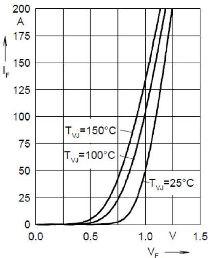
Fig. 1 Forward current I_F versus V_F
