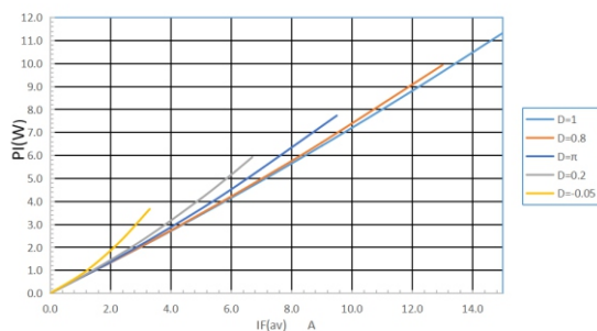
FIG.5- FORWARD POWER LOSS CHARACTERISTICS
