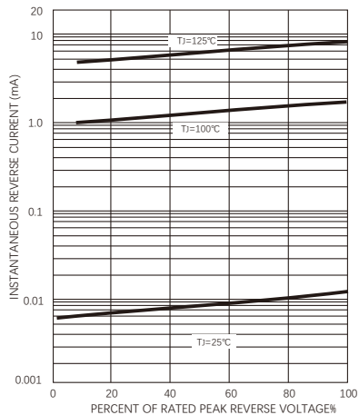
FIG.4-TYPICAL REVERSE CHARACTERISTICS
