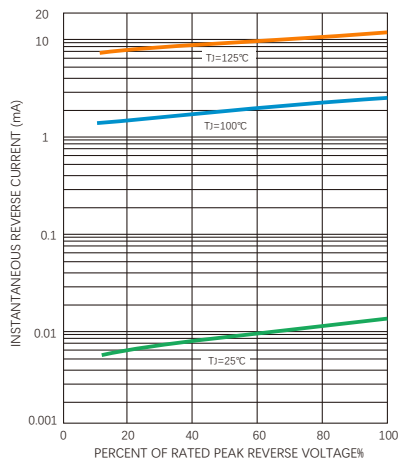
FIG.4-TYPICAL REVERSE CHARACTERISTICS
