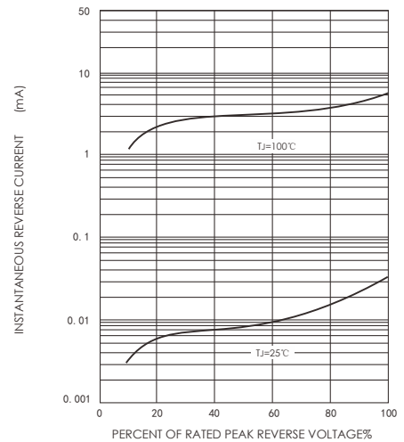
FIG.4-TYPICAL REVERSE CHARACTERISTICS
