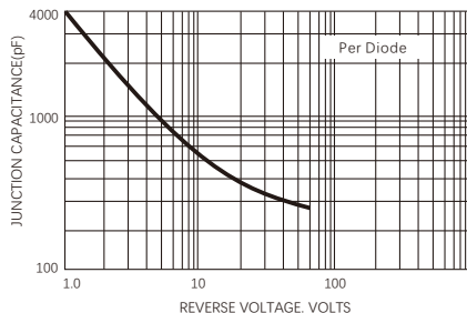
FIG.5-TYPICAL JUNCTION CAPACITANCE
