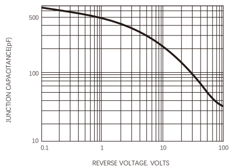
FIG.5-TYPICAL JUNCTION CAPACITANCE
