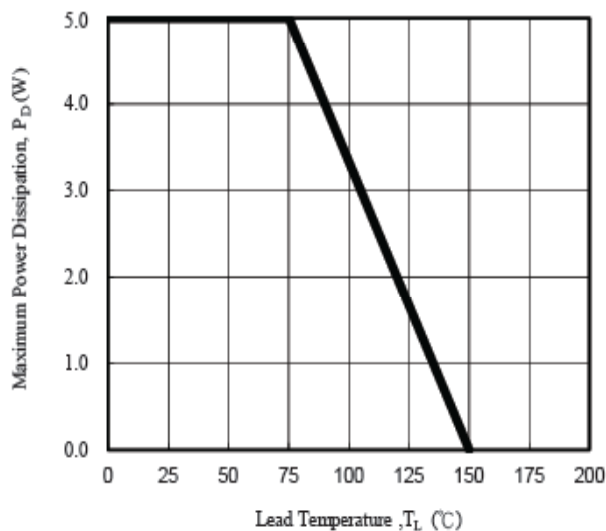
Fig. 1 - Power Temperature Derating Curve
