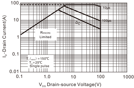
Fig7. Safe Operation Area
