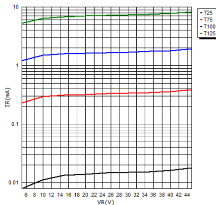
FIG.4-TYPICAL REVERSE CHARACTERISTICS
