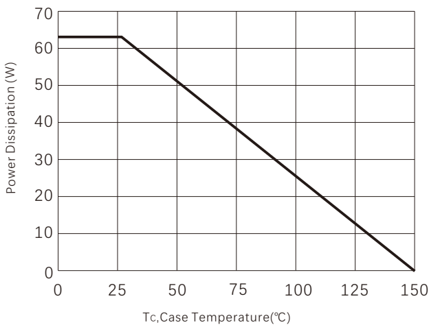
Figure 5. Power Dissipation
