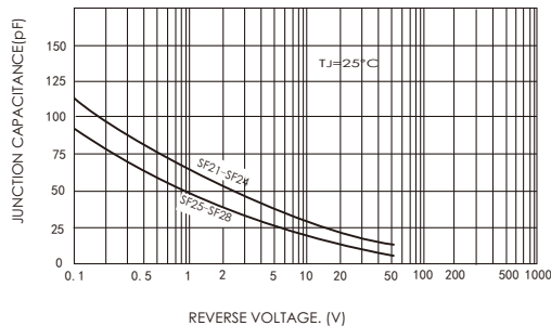
FIG.5-TYPICAL JUNCTION CAPACITANCE
