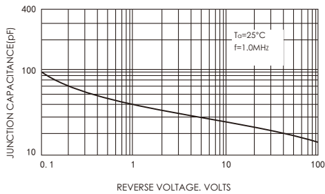
FIG.3-TYPICAL JUNCTION CAPACITANCE
