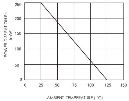
FIG.4-POWER DERATING CURVE
