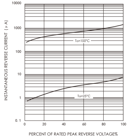
FIG.2-TYPICAL REVERSE CHARACTERISTICS
