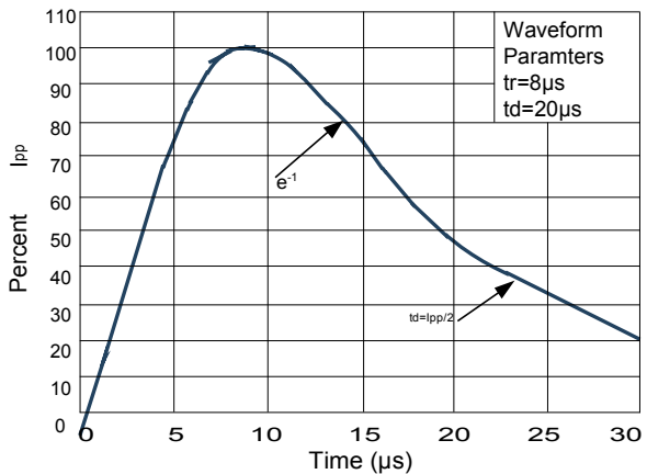
Figure3: Pulse Waveform
