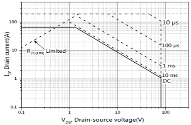
Figure8.Safe Operation Area
