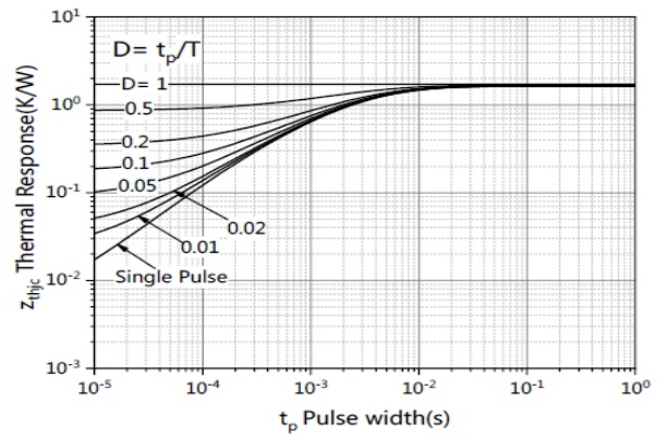
Figure10. Transient thermal impedance
