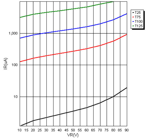
FIG.4-TYPICAL REVERSE CHARACTERISTICS
