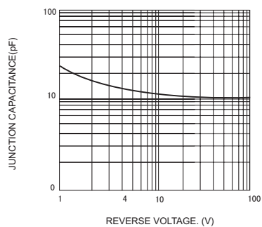
FIG3-TYPICAL JUNCTION CAPACITANCE
