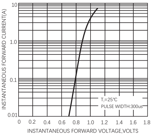
FIG. 3-TYPICAL FORWARD CHARACTERISTICS
