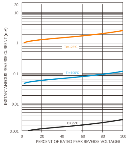
FIG.4-TYPICAL REVERSE CHARACTERISTICS
