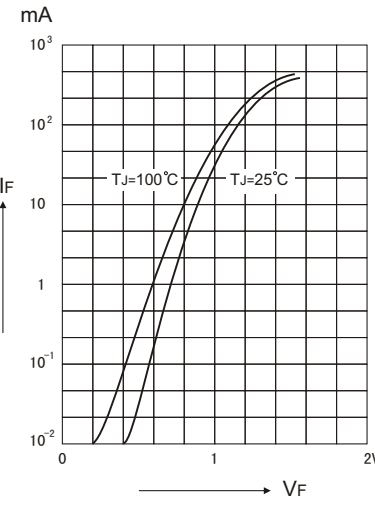
FIG 1-FORWARD CHARACTERISTICS
