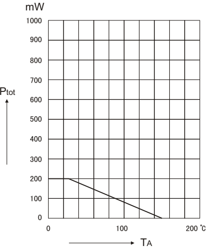
FIG 3-ADMISSIBLE POWER DISSIPATION VERSUS AMBIENT TEMPERATURE
